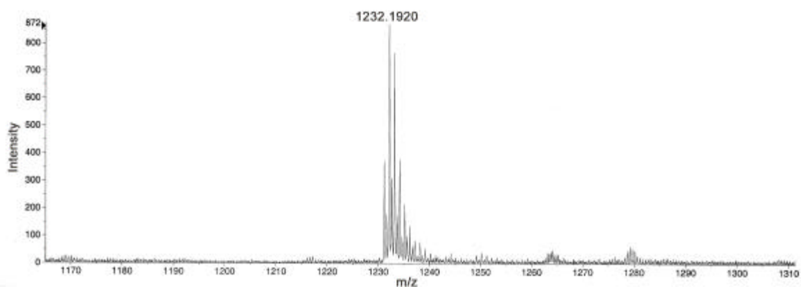
Figure S1. ESI mass spectrum of \text{Rh}_2(\text{DTolF})_2\{\text{d}(\text{GpA})\} collected in positive ion mode.
